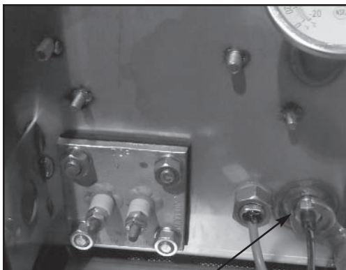
Removing the imperial brass fitting.
