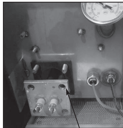
Pulling the heater out.
