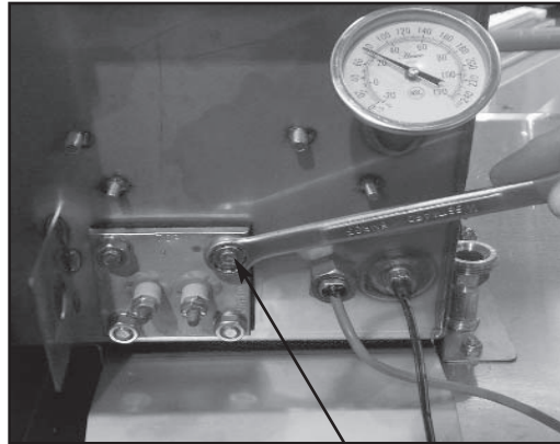
Removing the heater mounting nuts.
