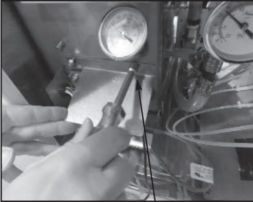
Removing the thermostat bracket.
